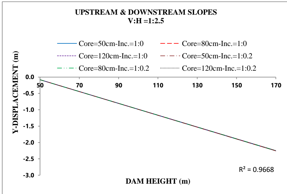
Figure 17. Vertical displacement diagram at the upstream top point in terms of dam height
