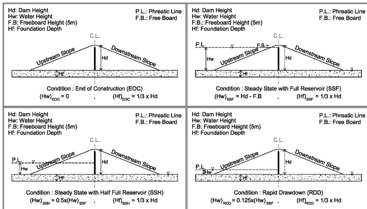
Figure 2. Different construction and impounding stages
