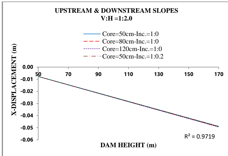
Figure 15. Horizontal displacement diagram at the upstream middle point in terms of dam height
