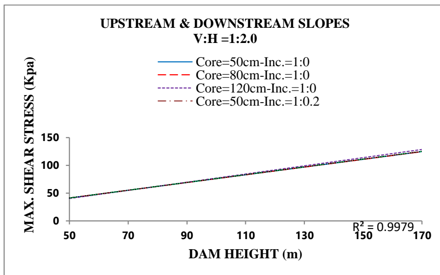
Figure 14. Maximum shear stress diagram at the upstream upper point in terms of dam height
