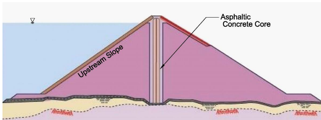
Figure 5. The Styggevatn Dam principal cross-section, located in Norway
