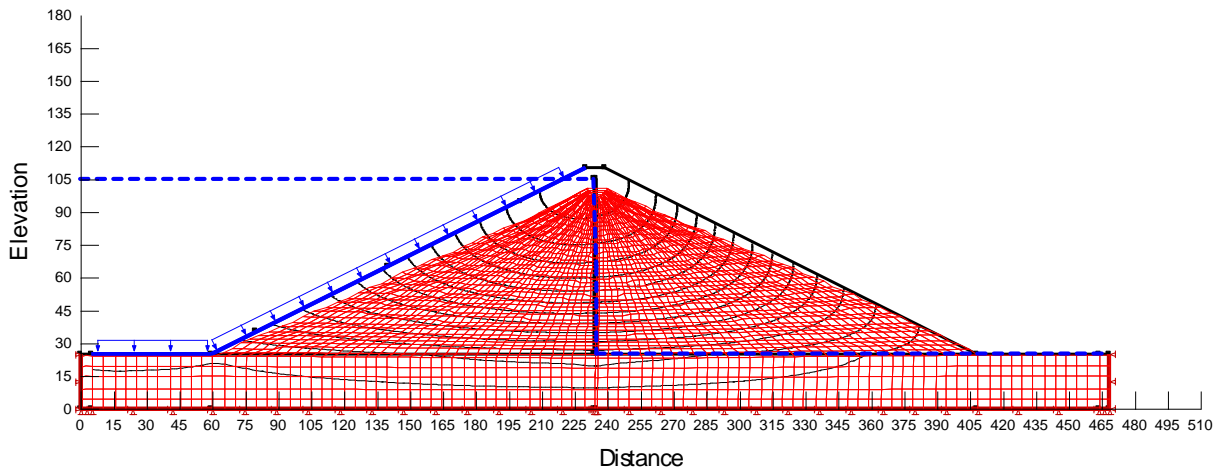
Figure 7. Vertical displacement vectors for height class 80 in full reservoir stage
