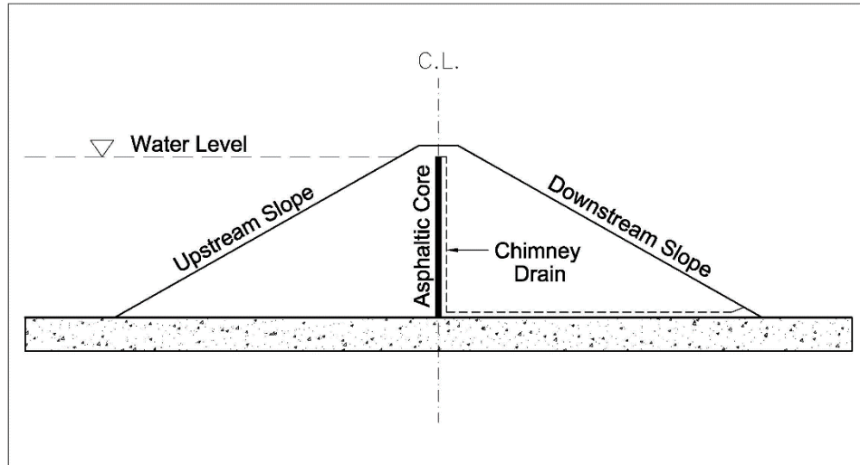
Figure 3. Chimney drain
