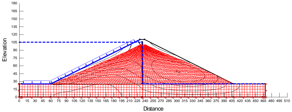
Figure 6. Horizontal displacement vectors for height class 80 in full reservoir stage
