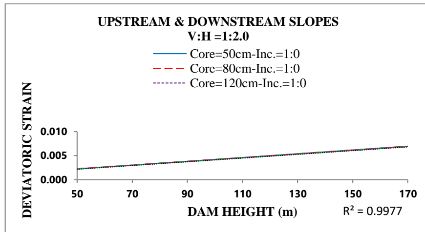
Figure 16. Maximum deviator strain diagram at the upstream lower point in terms of dam height
