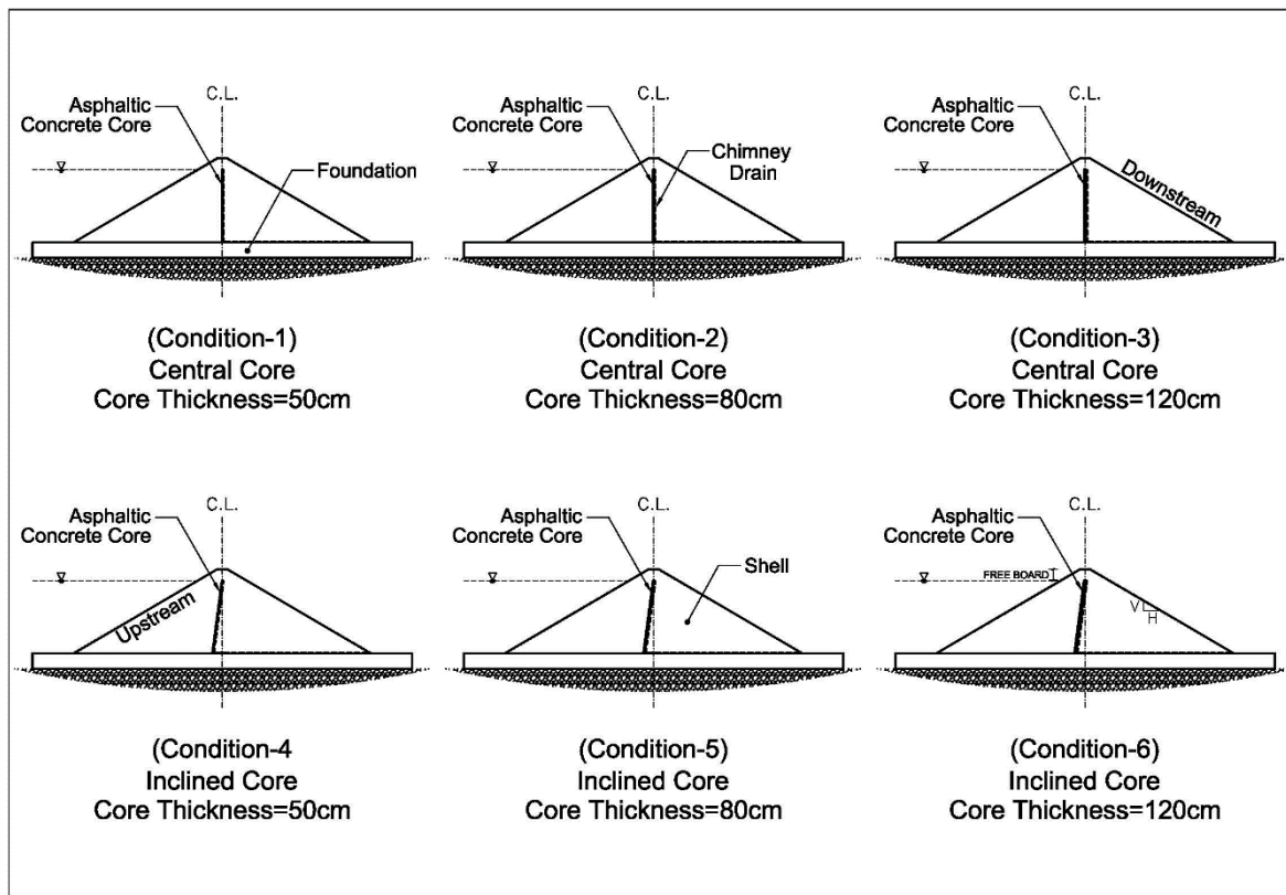
Figure 1. Thickness and the position of asphalt concrete core
