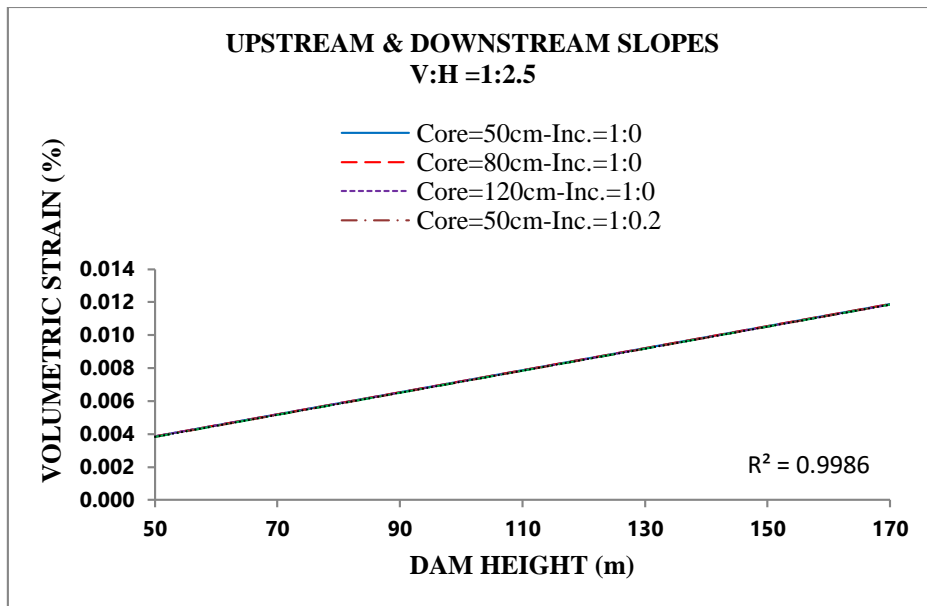
Figure 18. Volumetric strain diagram at the upstream bottom point in terms of dam height
