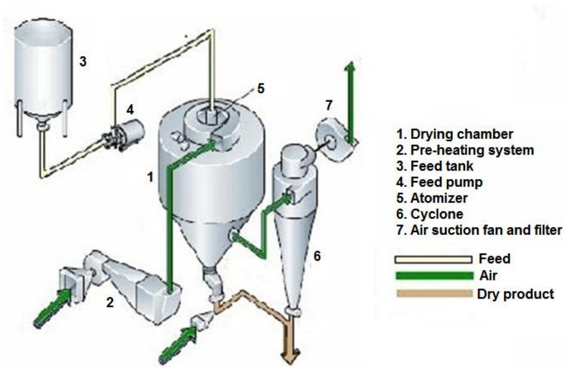
Figure 1. Diagram of the spray dryer used in this study. Source: Adapted from (Bylund, 1995)
