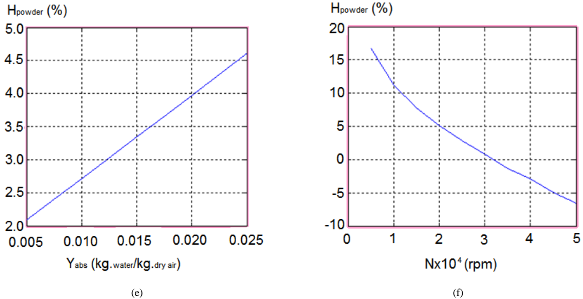
Figure 3. Relation of the final moisture of the powder with the following scale-up parameters: (a) Cream feed temperature. (b) Powder temperature. (c) Cream dry mass. (d) Air inlet temperature. (e) Absolute moisture of the air. (f) Synchronous speed of the atomizer disc.
