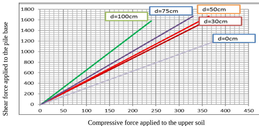
Figure 7. Base shear in piles
