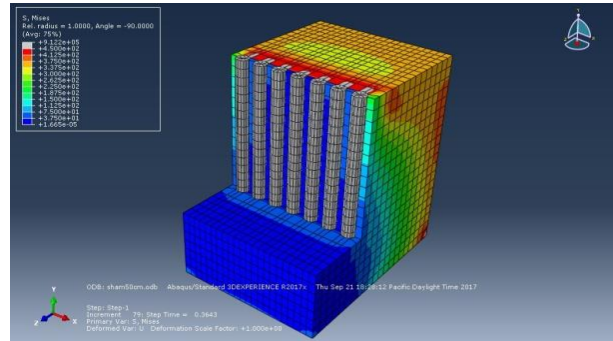
Pile distance is 75 cm
