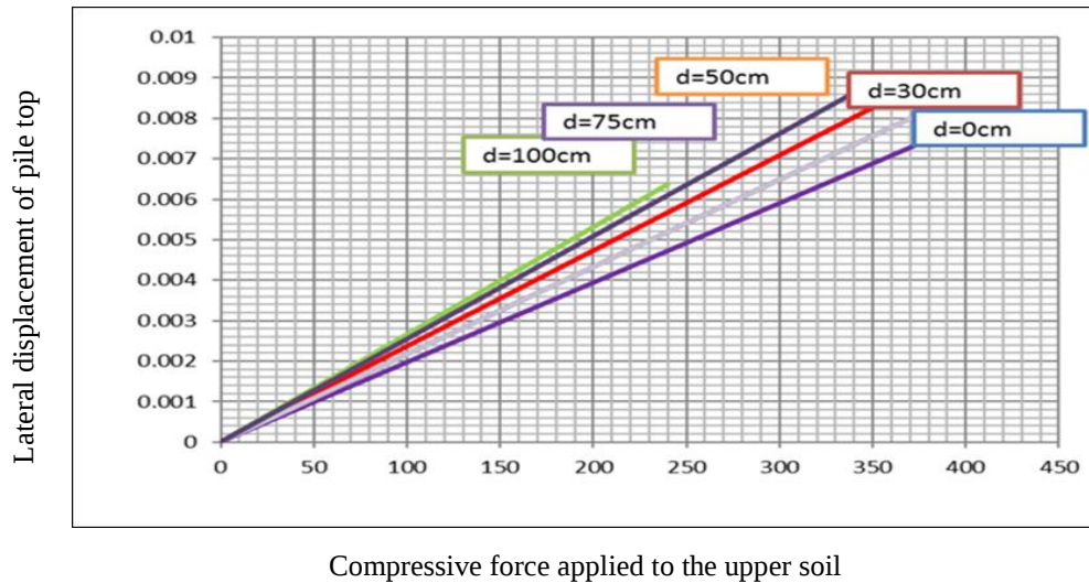
Figure 6. Piles lateral displacement
