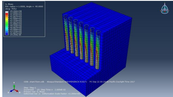
Pile distance is 50 cm
