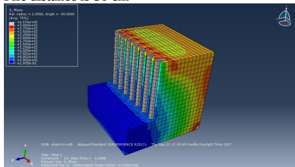
Pile distance is 100 cm
