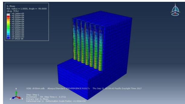
Pile distance is 30 cm
