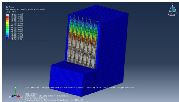
Pile distance is 0 cm
