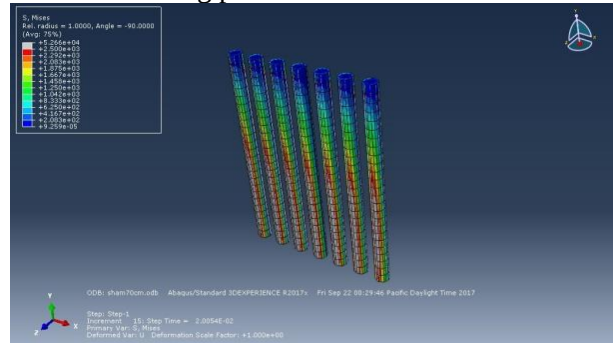
Distance among piles is 75 cm
